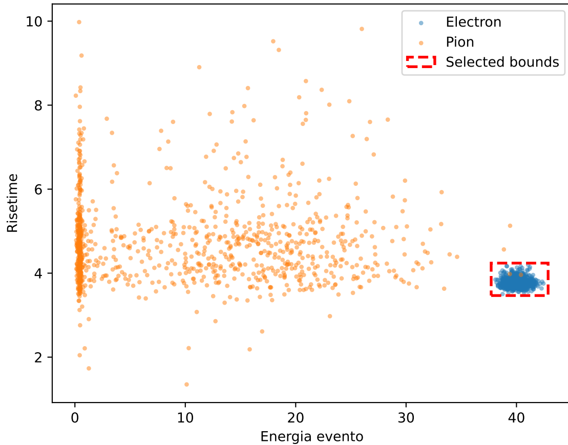
Scatter plot e/pi (all) 40.0GeV
