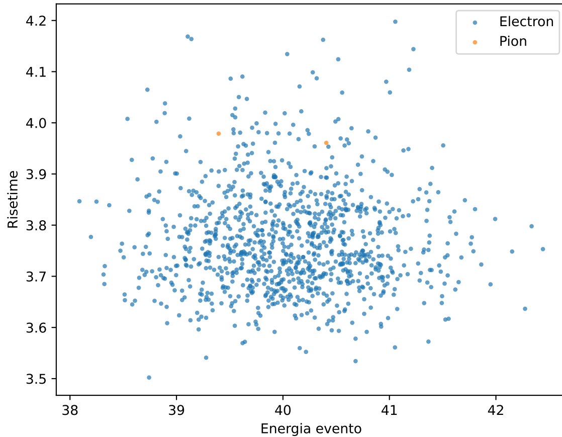
Scatter plot e/pi (cutted) 40.0GeV
